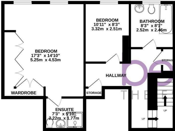
TOTAL FLOOR AREA : 1191 sq.ft. (110.7 sq.m.) approx.
